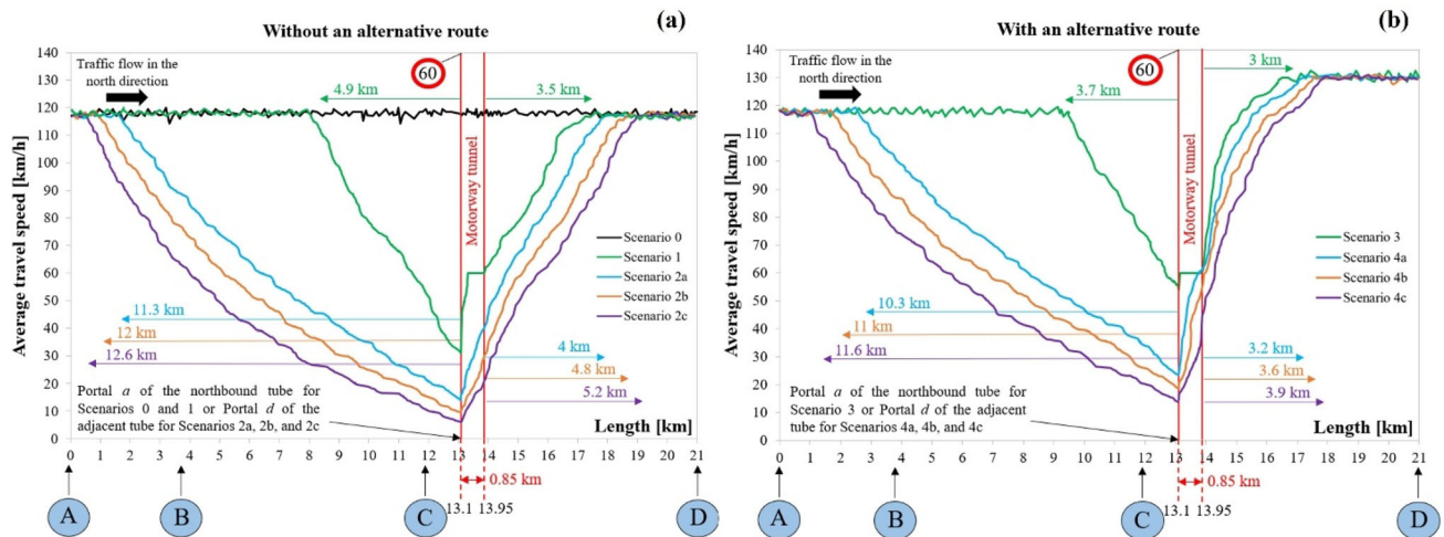
Fig. 6 Longitudinal spatial profiles of the average travel speed of the vehicular flow transiting along the motorway segment in the north direction (i.e., from the Nodes A to D) when the northbound tube is partially or completely closed for 2 h: a without an alternative route, b with an alternative route. Scenario 0 where the twin-tube motorway tunnel operates at its ordinary level of functionality; Scenario 1 in which the northbound tube is partially closed; Scenario 2 where the northbound tube is completely closed and the southbound tube is used for traffic in two driving directions through the opening of the traffic by-passes after 10 (Scenario 2a), 20 (Scenario 2b), or 30 min (Scenario 2c) from the occurrence of the disruptive event in the northbound tube; Scenario 3 that is similar to Scenario 1, but with only HGVs traveling northbound diverted along the alternative route; Scenarios 4a, 4b, and 4c that are similar to Scenarios 2a, 2b, and 2c, respectively, but with the activation of the alternative itinerary for only HGVs traveling along the motorway in the north direction
