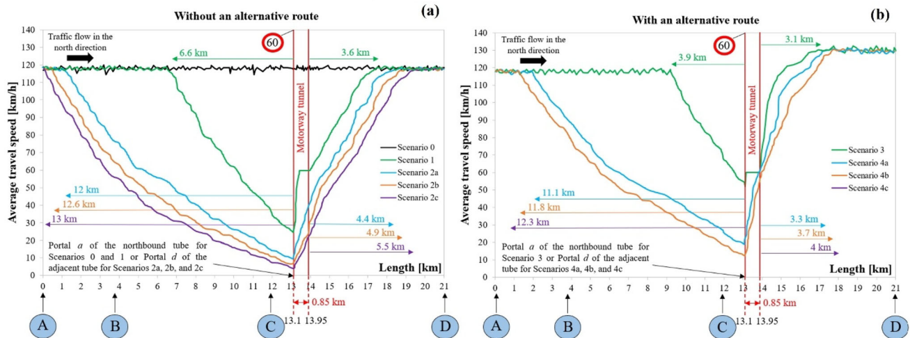
Fig. 7 Longitudinal spatial profiles of the average travel speed of the vehicular flow transiting along the motorway segment in the north direction (i.e., from the Nodes A to D) when the northbound tube is partially or completely closed for 3 h: a without an alternative route, b with an alternative route. Scenario 0 where the twin-tube motorway tunnel operates at its ordinary level of functionality; Scenario 1 in which the northbound tube is partially closed; Scenario 2 where the northbound tube is completely closed and the southbound tube is used for traffic in two driving directions through the opening of the traffic by-passes after 10 (Scenario 2a), 20 (Scenario 2b), or 30 min (Scenario 2c) from the occurrence of the disruptive event in the northbound tube; Scenario 3 that is similar to Scenario 1, but with only HGVs traveling northbound diverted along the alternative route; Scenarios 4a, 4b, and 4c that are similar to Scenarios 2a, 2b, and 2c, respectively, but with the activation of the alternative itinerary for only HGVs traveling along the motorway in the north direction
