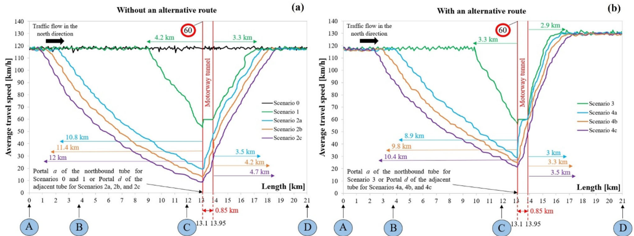
Fig. 5 Longitudinal spatial profiles of the average travel speed of the vehicular flow transiting along the motorway segment in the north direction (i.e., from the Nodes A to D) when the northbound tube is partially or completely closed for 1 h: a without an alternative route, b with an alternative route. Scenario 0 where the twin-tube motorway tunnel operates at its ordinary level of functionality; Scenario 1 in which the northbound tube is partially closed; Scenario 2 where the northbound tube is completely closed and the southbound tube is used for traffic in two driving directions through the opening of the traffic by-passes after 10 (Scenario 2a), 20 (Scenario 2b), or 30 min (Scenario 2c) from the occurrence of the disruptive event in the northbound tube; Scenario 3 that is similar to Scenario 1, but with only HGVs traveling northbound diverted along the alternative route; Scenarios 4a, 4b, and 4c that are similar to Scenarios 2a, 2b, and 2c, respectively, but with the activation of the alternative itinerary for only HGVs traveling along the motorway in the north direction
